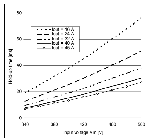
Hold-up time (min., at V_{out}=24V )
