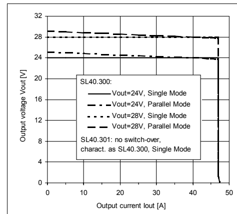
Output V/I characteristic (typ.)
