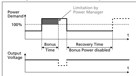
Fig. 6-5 BonusPower® recovery time
