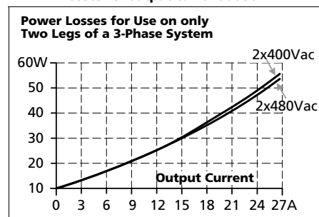
Losses vs. output current at 36V
