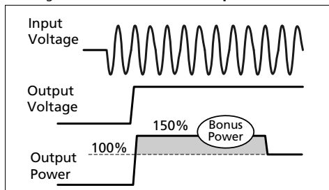
Fig. 6-6 BonusPower® after input turn-on
