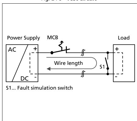
Fig. 24-9 Test circuit
