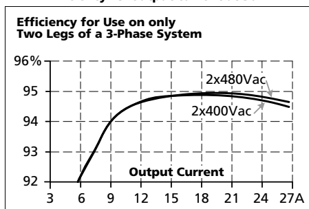
Efficiency vs. output current at 36V
