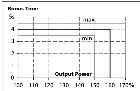
Fig. 6-3 Bonus time vs. output power
