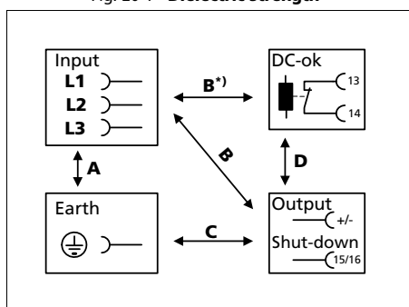
Fig. 20-1 Dielectric strength
