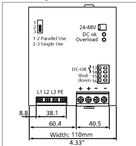
Fig. 22-1 Front view
