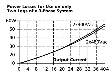
Losses vs. output current at 24V
