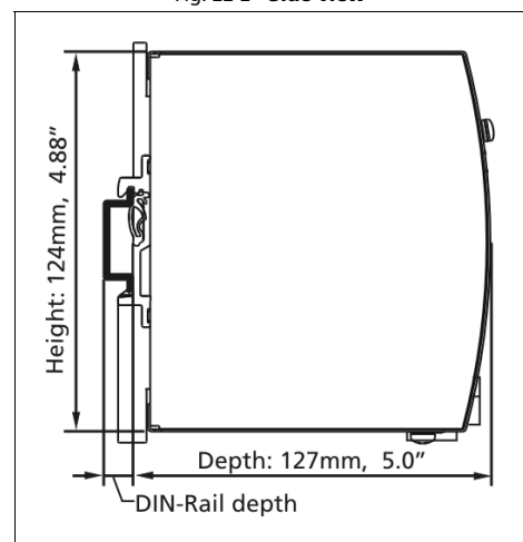
Fig. 22-2 Side view
