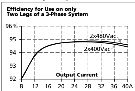
Efficiency vs. output current at 24V
