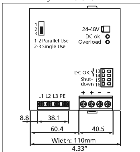
Fig. 22-1 Front view
