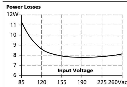
Fig. 9-4 Losses vs. input voltage at 3.8A, typ.
