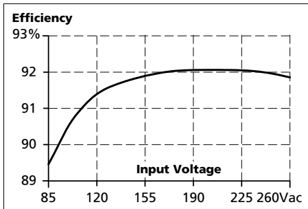
Fig. 9-3 Efficiency vs. input voltage at 3.8A, typ.
