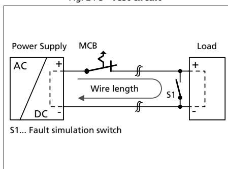
Fig. 24-3 Test circuit
