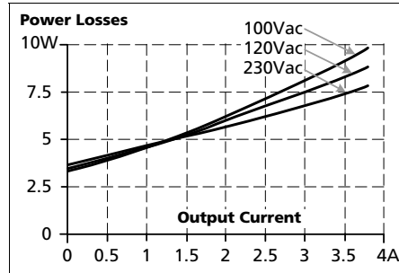
Fig. 9-2 Losses vs. output current, typ.
