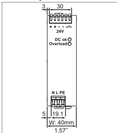
Fig. 22-1 Front view
