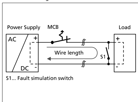
Fig. 24-5 Test circuit
