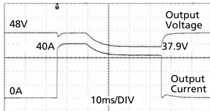
Fig. 25-3 Peak load with 2x the nominal current for 50ms, typ.
