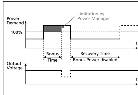
Fig. 6-6 BonusPower ® recovery time
