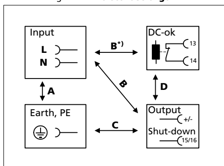
Fig. 21-1 Dielectric strength
