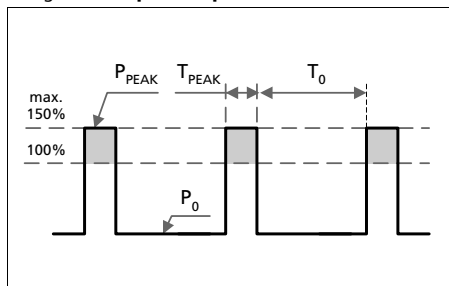
Fig. 23-1 Repetitive pulse loads, definitions
