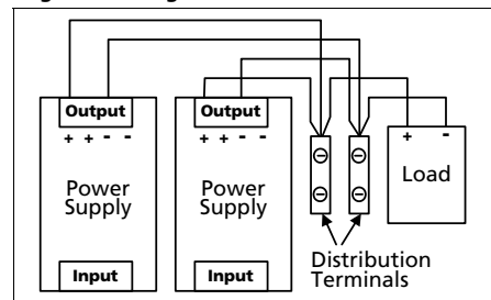
Fig. 23-6 Using distribution terminals
