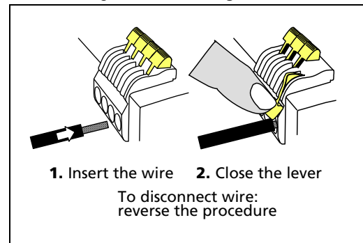
Fig. 11-1 Connecting a wire
