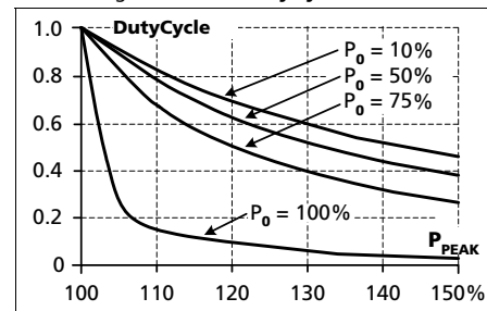
Fig. 23-2 Max. duty cycle curve
