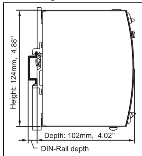
Fig. 21-2 Side view
