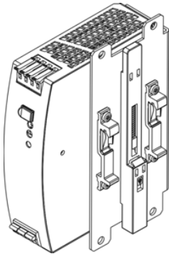
Side mounting with DIN-rail brackets
