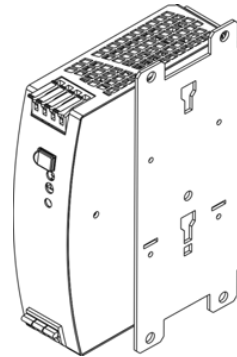
Side mounting without DIN-rail brackets
