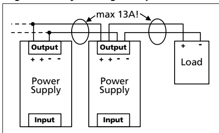
Fig. 23-5 Daisy chaining of outputs
