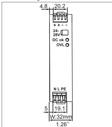
Fig. 21-1 Front view
