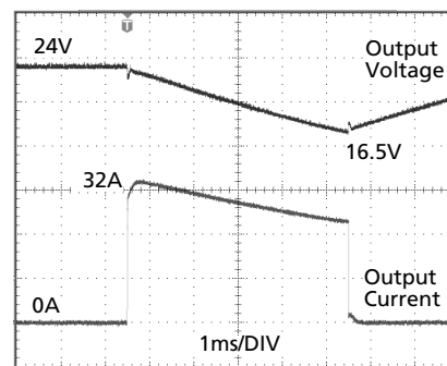
Fig. 22-2 Peak load with 4x the nominal current for 5ms, typ.
