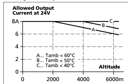
Fig. 15-2 Output current vs. altitude
