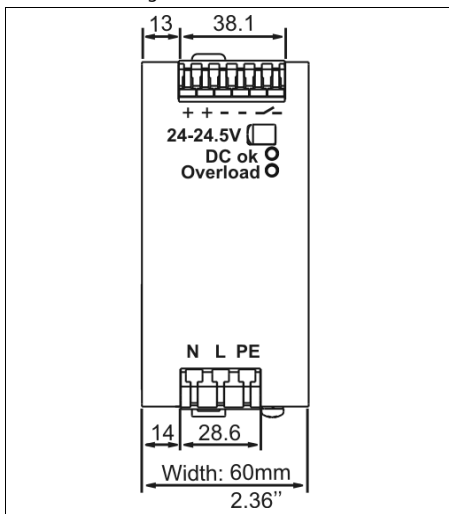
Fig. 20-1 Front view
