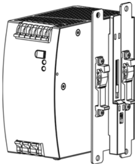
Side mounting with DIN-rail brackets
