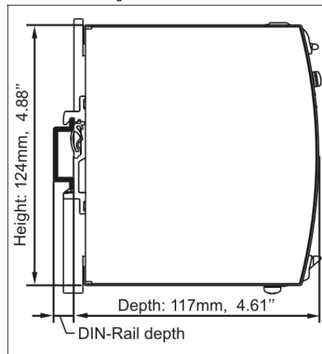
Fig. 20-2 Side view
