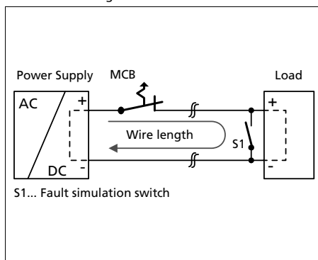
Fig. 22-3 Test circuit
