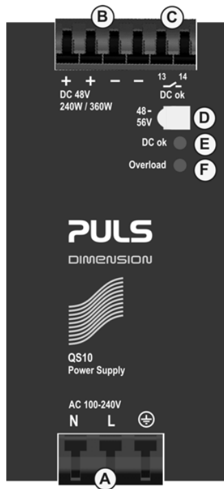
Fig. 13-1 Front side
