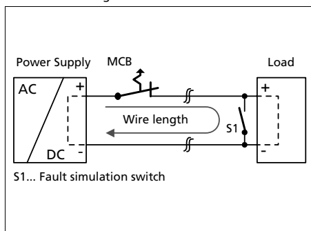
Fig. 22-5 Test circuit
