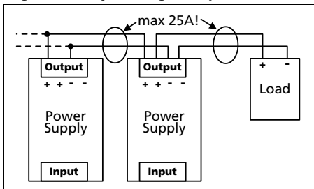
Fig. 24-6 Daisy chaining of outputs
