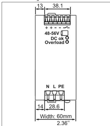
Fig. 22-1 Front view
