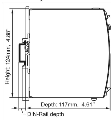
Fig. 22-2 Side view
