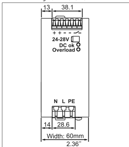
Fig. 20-1 Front view
