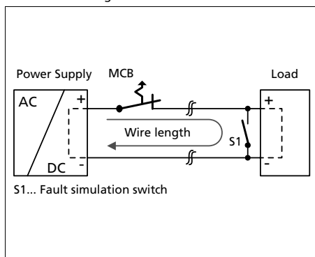
Fig. 22-5 Test circuit
