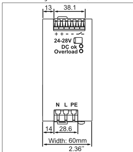
Fig. 20-1 Front view
