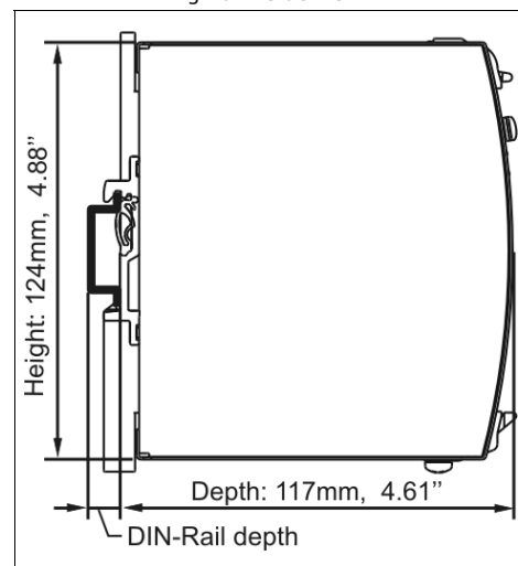
Fig. 20-2 Side view
