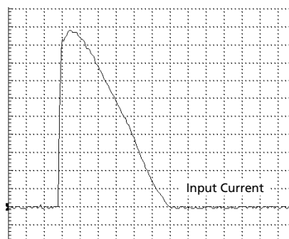
Fig. 4-2 Input inrush current, zoom into first peak
