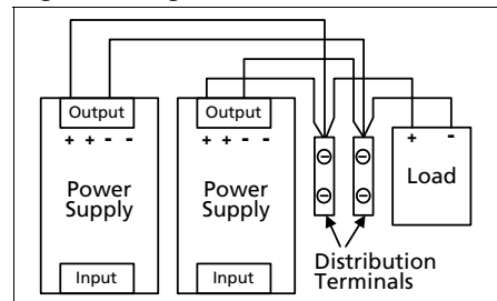
Fig. 22-4 Using distribution terminals
