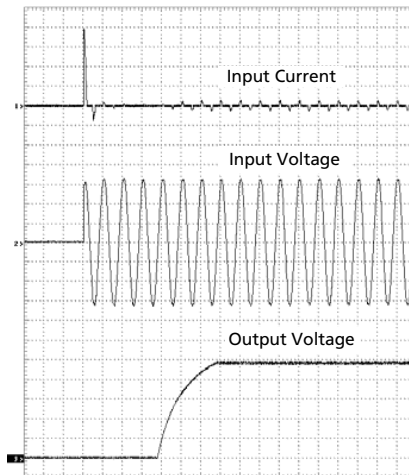
Fig. 4-1 Input inrush current, typical behavior
