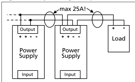
Fig. 22-3 Daisy chaining of outputs
