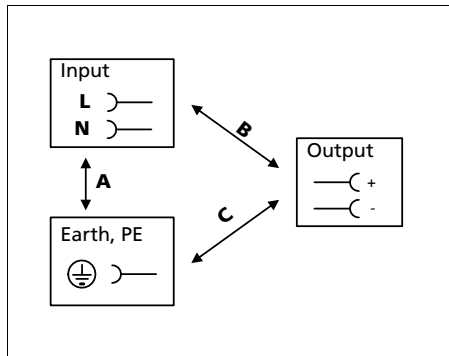
Fig. 17-1 Dielectric strength
