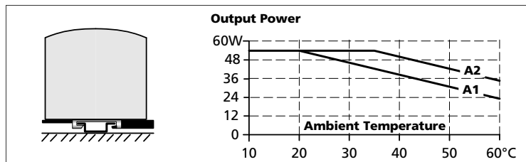
Fig. 22-9 Mounting Orientation C (Table-top mounting)
