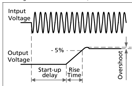
Fig. 5-2 Turn-on behavior, definitions
