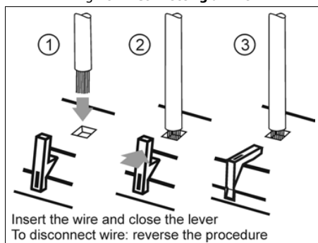
Fig. 15-1 Connecting a wire
