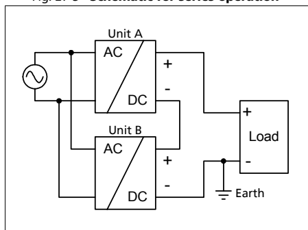
Fig. 27-3 Schematic for series operation
