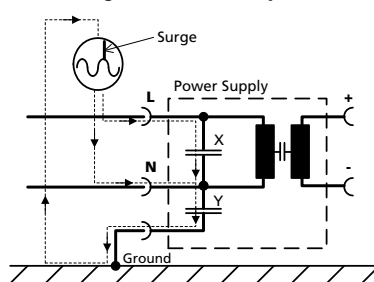
Fig. 22-3 Earthed input
