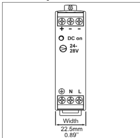
Fig. 20-1 Front view
