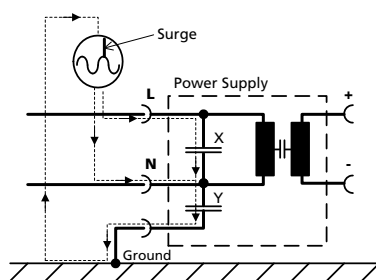
Fig. 22-3 Earthed input
