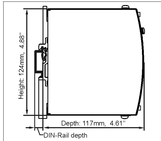
Fig. 20-2 Side view
