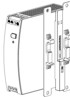
Side mounting without DIN-rail brackets
