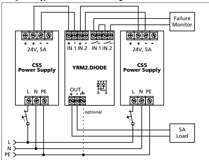
Fig. 21-1 Typical 1+1 Redundant configuration for 5A load current
