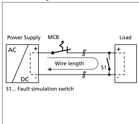
Fig. 22-3 Test circuit
