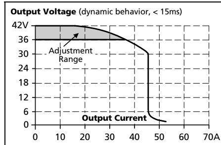
Fig. 6-4 Dynamic overcurrent capability, typ.
