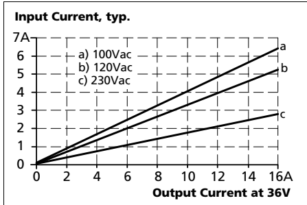
Fig. 3-3 Input current vs. output current
