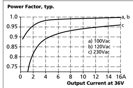
Fig. 3-4 Power factor vs. output current
