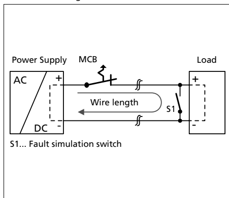
Fig. 24-4 Test circuit
