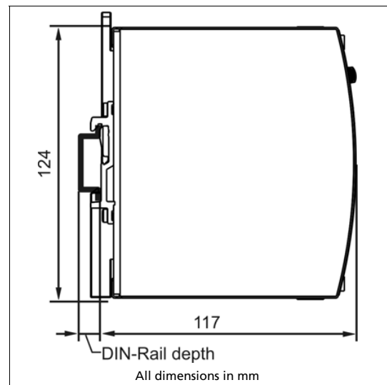
Fig. 22-2 Side view
