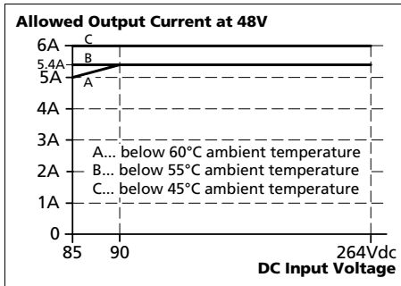
Fig. 3-5 Derating requirements
