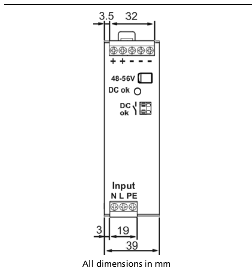
Fig. 22-1 Front view
