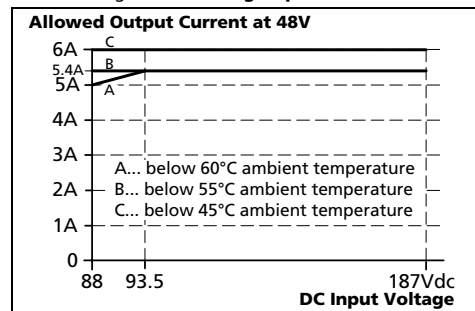
Fig. 4-2 Derating requirements
