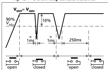
Fig. 12-1 DC-ok relay contact behavior
