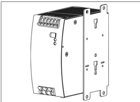
Fig. 22-3 ZM11.SIDE Side mounting bracket *)
