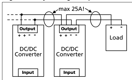
Fig. 23-4 Daisy chaining of outputs
