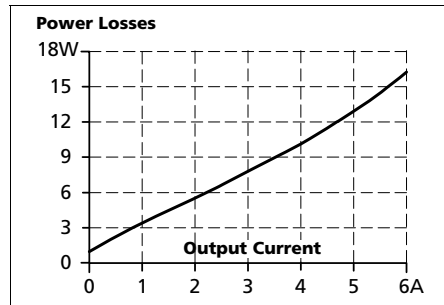
Fig. 7-2 Losses vs. output current at 24V, typ.
