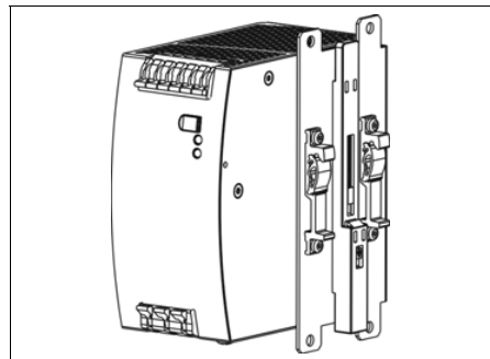
Fig. 22-4 Side mounting with DIN-rail brackets *)
