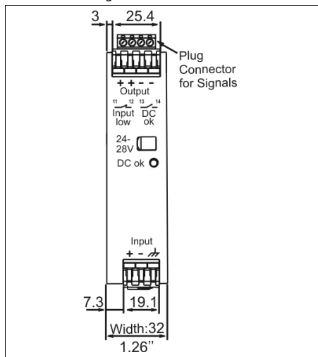
Fig. 21-1 Front view
