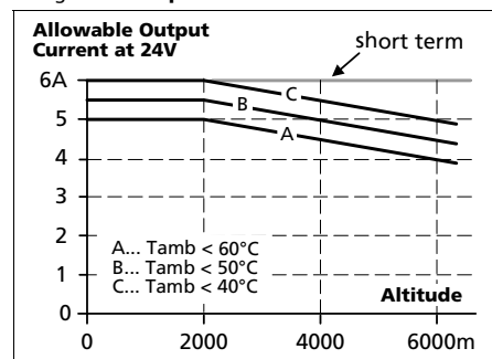
Fig. 15-2 Output current vs. altitude at 24V
