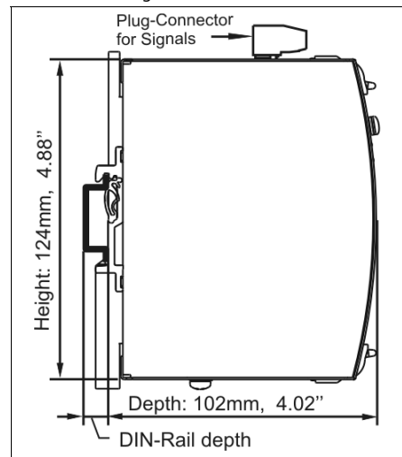
Fig. 21-2 Side view
