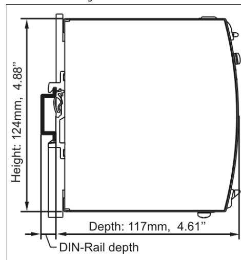
Fig. 22-2 Side view
