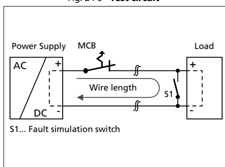
Fig. 24-5 Test circuit
