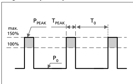
Fig. 24-1 Repetitive pulse loads, definitions
