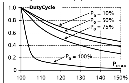
Fig. 24-2 Max. duty cycle curve
