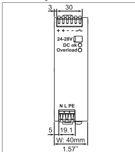
Fig. 22-1 Front view
