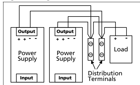
Fig. 24-7 Using distribution terminals
