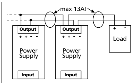
Fig. 24-6 Daisy chaining of outputs
