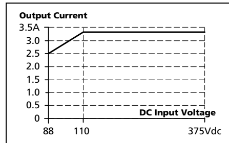
Fig. 4-2 Output current vs. input voltage
