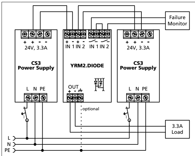
Fig. 21-1 Typical 1+1 Redundant configuration for 3.3A load current
