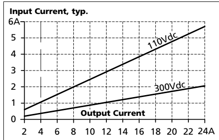
Fig. 4-3 Input current vs. output load at 24V
