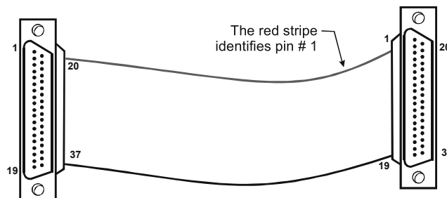
Figure 3. C37FF-x cable
