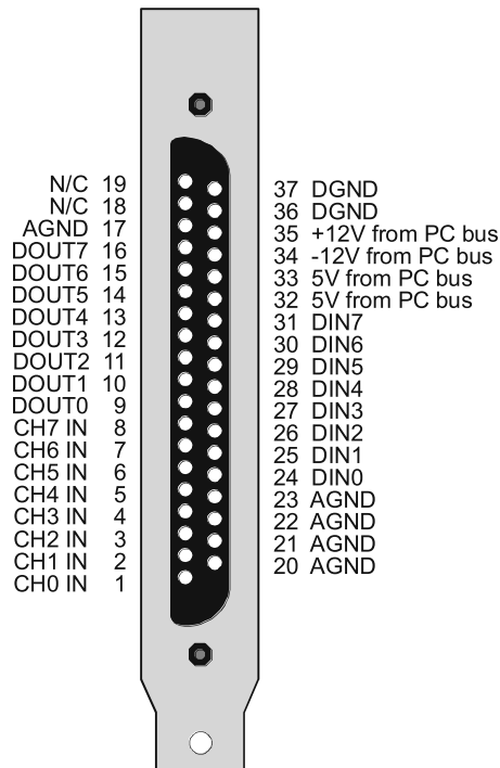
Figure 2. CIO-DAS08/JR pin-out
